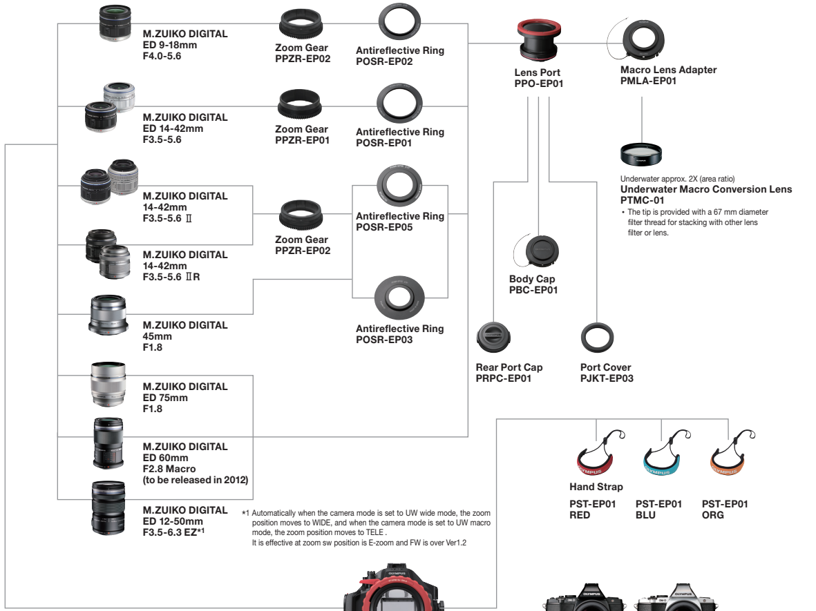
Underwater Case for OM-D PT-EP08
